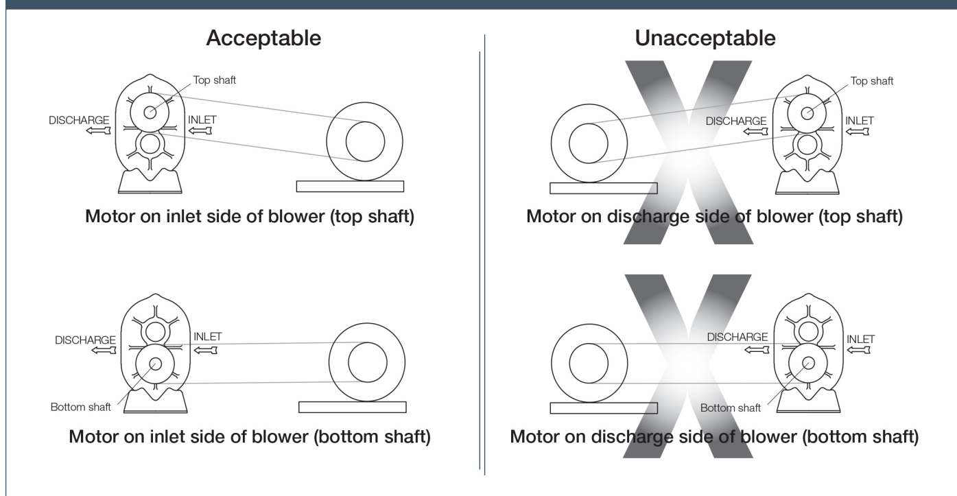
Figure 1 – Acceptable blower drive arrangement options
